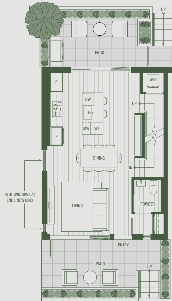
MAIN - LEVEL 1
